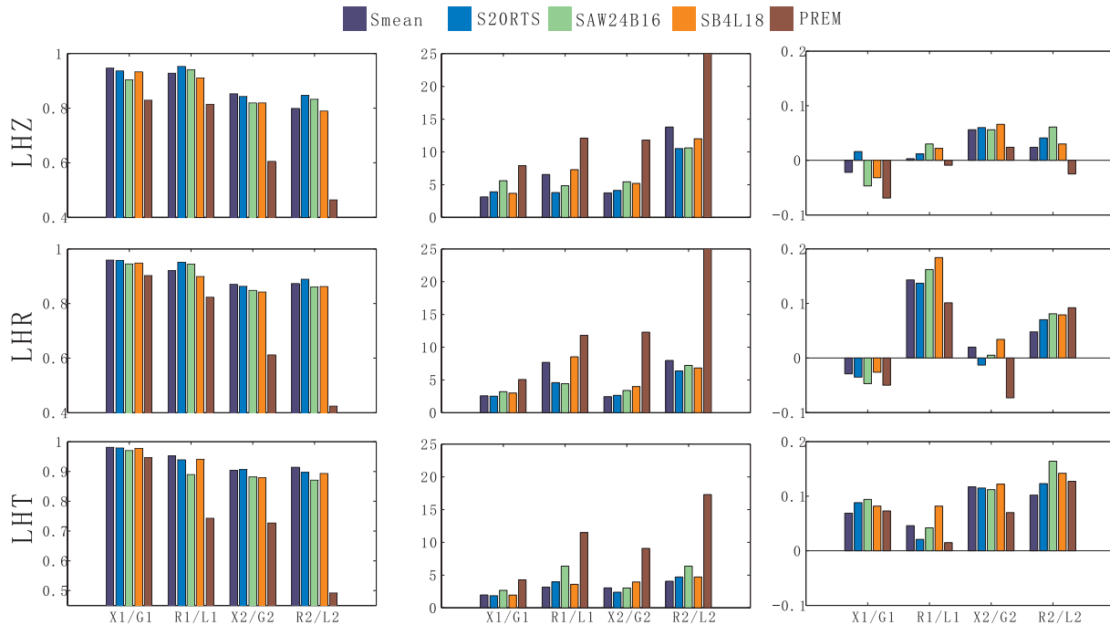
Figure 9. The average correlation coefficients (left column), time lag (middle column) and amplitude ratio (right column) for different components (R1, R2, X1 and X2 for vertical and longitudinal components; L1, L2, G1 and G2 for transverse component), different tomographic models and different time windows for a deep event (645 km deep) located in eastern Russian–northeastern China border which occurred on 2002 June 28. L1, minor-arc fundamental Love train; L2, major-arc fundamental Love train; R1, minor-arc fundamental Rayleigh train; R2, major-arc fundamental Rayleigh train; G1, minor-arc higher-mode Love train; G2, major-arc higher-mode Love train; X1, minor-arc higher-mode Rayleigh train; X2, major-arc higher-mode Rayleigh train. The results clearly demonstrated that the agreement in the phase between observations and synthetics is significantly improved by 3-D tomographic models by comparing with PREM model, but not in the amplitude. For the amplitude ratio in the right column, the value 1.0 has been removed.
