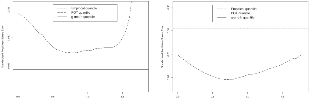
FIGURE 5: SRMSE for the “soft” case (left panel) and for the “hard” case (right panel).
