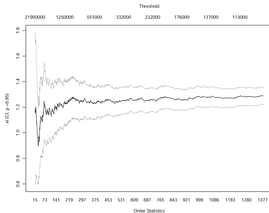
FIGURE 4: Hill plot for g = 4, h = 0.2 and n = 10^6 .
