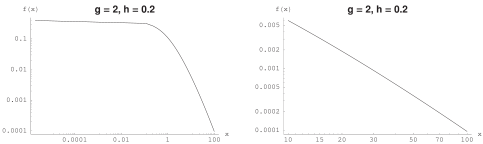
FIGURE 2: Density of the g-and-h distribution plotted on a log-log scale. Note the different plotting ranges of the axes.
