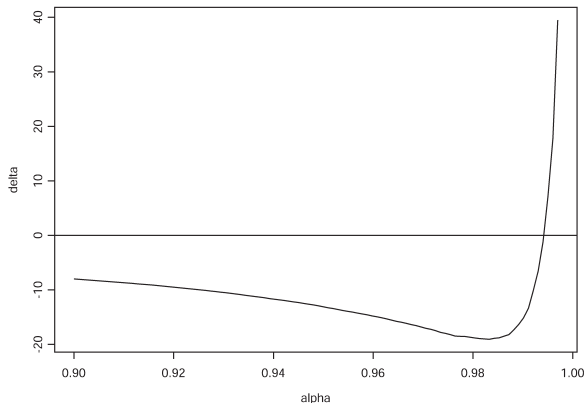
FIGURE 6: Plot of \delta_{g,h}(\alpha) as a function of \alpha for g = 2.4 , h = 0.2 ; n = 10^7 .
