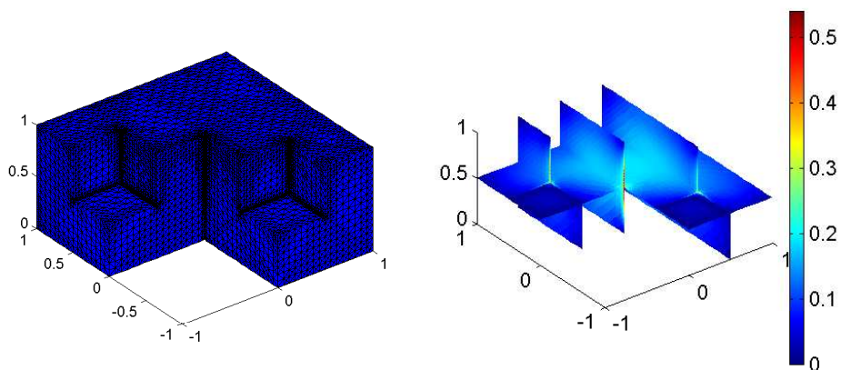
Figure 5: The mesh plot and the slice plot of the the amplitude of the discrete solution for Example 7.2 after 24 local refinements. The mesh contains 258,849 tetrahedrons.
