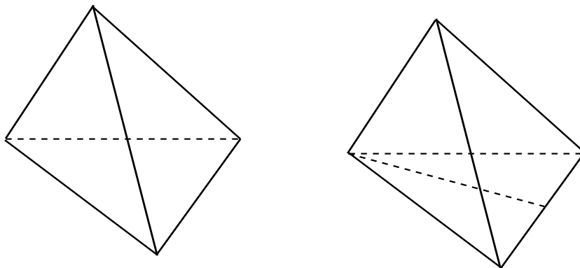
Figure 1: Left: A tetrahedron to be refined. Right: The tetrahedron is bisected into two tetrahedrons. The smoothed vertices are the new vertex and the two endpoints of the refinement edge (two “immediately neighboring vertices”). The smoothing edges are the four new edges and the old edges of the two faces which share the refinement edge (“immediate neighboring edges” of the centerlines).
