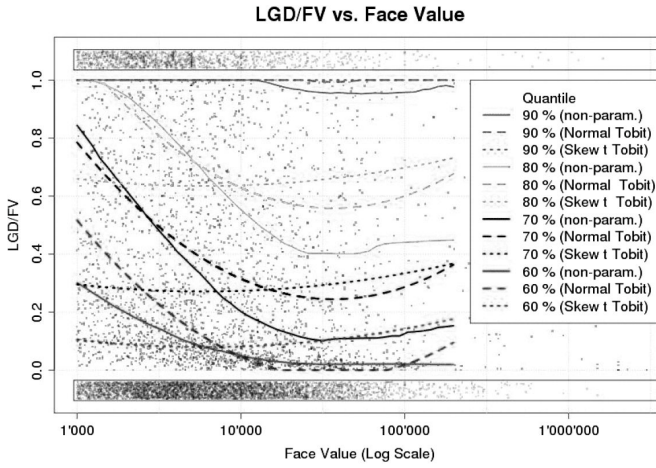
FIGURE 5: Scatter plot of LGD/FV versus face value (on a logarithmic scale).
