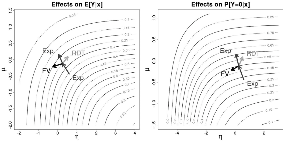
FIGURE 3: Illustration of effects of main covariates for the zero-inflated model. On the left hand side, a contour plot of the conditional expectation, E[Y|\mathbf{x}] , as a function of the two linear predictors \eta = \mathbf{x}'\boldsymbol{\beta} and \mu = \mathbf{x}'\boldsymbol{\gamma} is shown. On the right hand side, the same contour plot is shown for the probability of being zero, P[Y = 0|\mathbf{x}] . The arrows represent the effects of changing covariates. For the two continuous covariates face value (FV) and relative default time (RDT), the arrows are obtained by increasing the variables by one standard deviation from their mean. For the factorial variable experience (Exp), the two arrows indicate the changes when moving from the lowest level to the middle one and then to the highest level.
