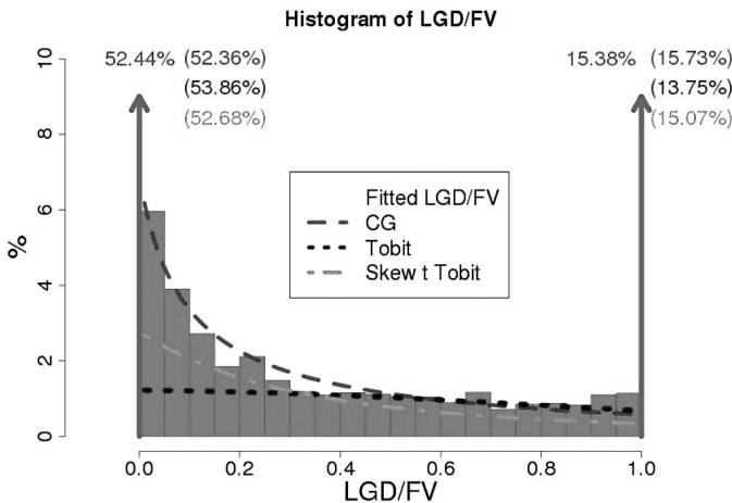
FIGURE 4: Comparison of fitted censored gamma, normal Tobit, and skew t Tobit models with no covariates. The numbers above the blue arrows represent the percentage of LGD/FV's being exactly zero or one, respectively. In parentheses are the corresponding numbers as predicted by the models.
