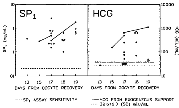
Figure 1. Detection of implantation by serum pregnancy-specific \beta 1-glycoprotein (SP 1 ) and human chorionic gonadotrophin (HCG). Individual readings obtained between the day of oocyte retrieval+13 and the day of oocyte retrieval+19 for 'interaction' group (IC; no ongoing pregnancy, open circles) and clinical pregnancy group (CP; filled circles). Two patients assayed twice are shown by pairs of points joined by solid lines.
