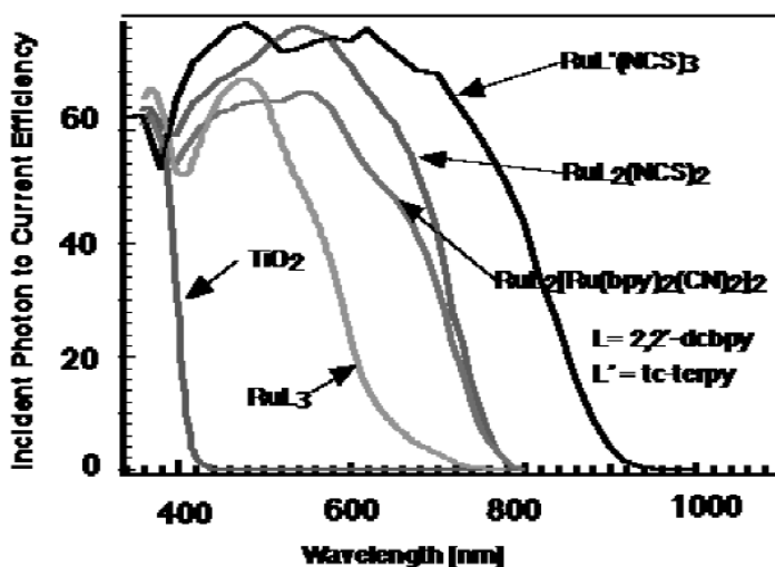
Fig. 5 Photocurrent action spectrum of bare nanocrystalline \text{TiO}_2 films and sensitized by various ruthenium complexes, the conversion efficiency of incident photons to electric current is plotted as a function of the excitation wavelength.
