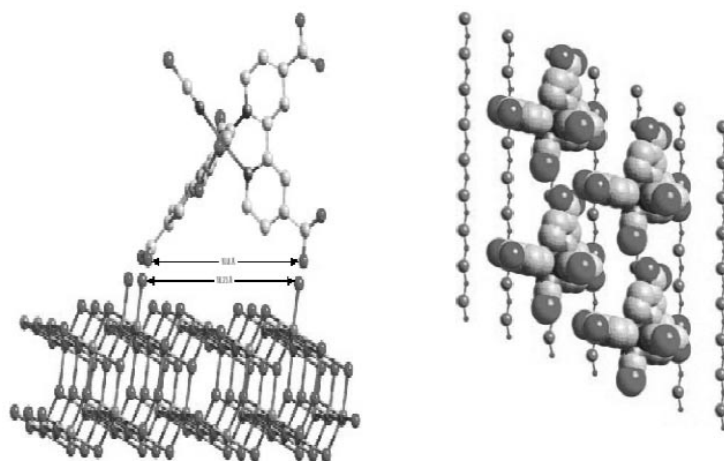
Fig. 4 Structural presentation of the N3 ruthenium complex adsorbed onto the (101) surface of anatase. Left: side view; right: top view.
