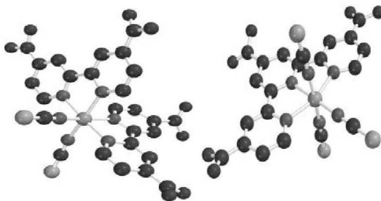
Fig. 3 Structure of cis -dithiocyanato-bis(2,2'-bipyridyl-4,4'-dicarboxylate)-ruthenium(II), RuL_2(SCN)_2 (left) and the black dye Ru(tcterypy)(SCN)_3 , tcterypy = 4,4',4'' -tricarboxy-2,2':6,2''-terpyridine.
