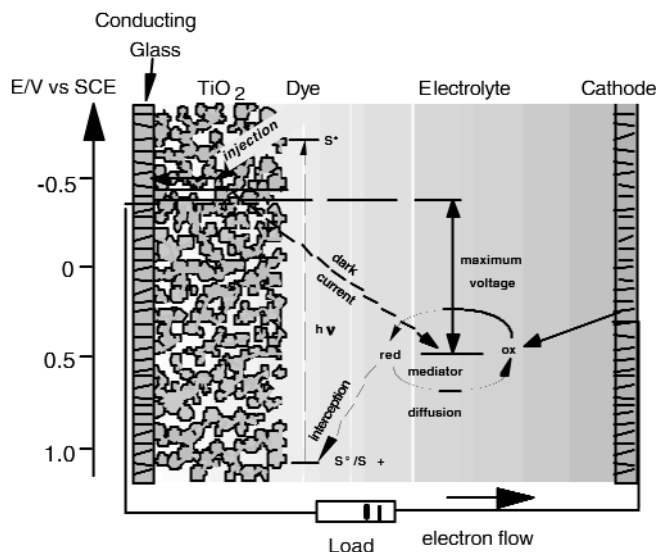
Fig. 1 Biomimetic conversion of light to electricity using two redox catalytic cycles. As in natural photosynthesis, in the artificial analog sunlight sets in action a molecular electron pump. The sensitizer (S) is bound as a monomolecular coating on the surface of a semiconductor oxide, such as TiO 2 , ZnO, SnO 2 or Nb 2 O 5 . It absorbs the incident solar rays, and is thereby raised to the electronically excited state S*. From this state it injects an electron into the conduction band of the oxide. The conduction band electrons then cross the film and are directed through a charge collector into the external current circuit where electrical work is done. The electrons are then returned to the cell through a counter electrode. Between this counter electrode and the oxide is an electrolyte containing a redox couple, i.e., iodine and iodide. This redox electrolyte allows for the transport of electrical charge between the two electrodes. The electrons reduce triiodide to iodide ions which diffuse from the counter electrode to the nanocrystalline film surface where they regenerate the sensitizer by electron transfer to the sensitizer cations, while simultaneously the iodide is oxidized back to iodine or triiodide. The redox catalytic cycle leading to the conversion of light into electrical current is thereby closed.
