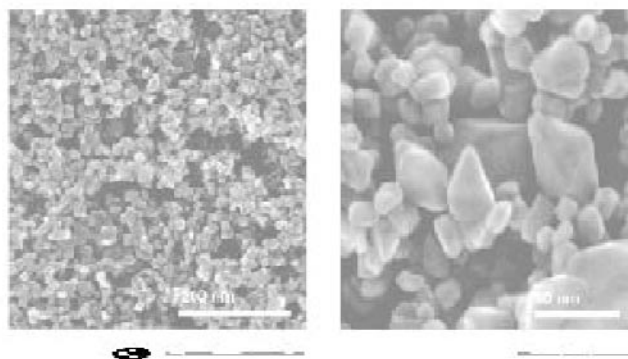
Fig. 2 Scanning electron microscope picture of a nanocrystalline titania (anatase) film.
