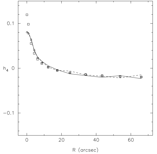
Figure 7. Seeing convolution test, comparing the radial run of h_4 along a 2-arcsec slit for a spherical target model and its particle representation. The squares (circles) were computed for the target from higher order Jeans equations without (with) seeing. The lines correspond to the particle model including seeing, for which the PSF was represented using N_{pp} = 5 . The full and dashed lines refer to the major-axis slit data at, respectively, positive and negative radii with respect to the origin. The heavily seeing-affected central profile is well recovered by the model.
