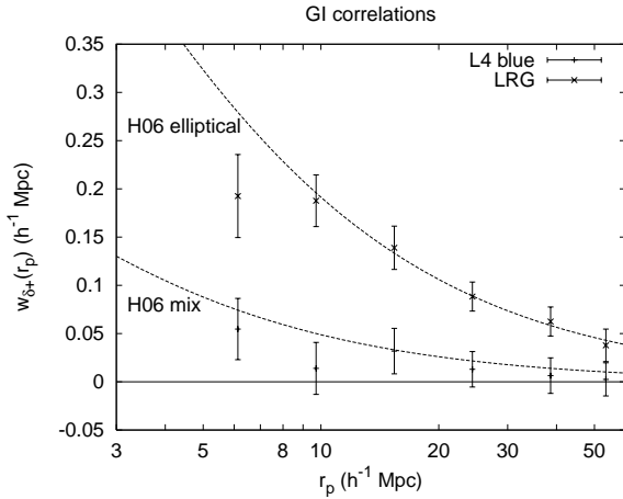
Figure 9. The GI correlation functions w_{\delta+}(r_p) for the full SDSS LRG sample and the L4 blue sample, with the galaxy-to-density conversion using biases of 1.99 and 1.12, respectively. The lines are the curves from Heymans et al. (2006b) at z = 0.27 , interpreted using the procedure in Appendix B. The median redshift of the LRGs is z_{\text{med}} = 0.27 ; the L4 blue galaxies have z_{\text{eff}} = 0.12 , although we expect that evolution between 0.12 and 0.27 would make a small effect.
