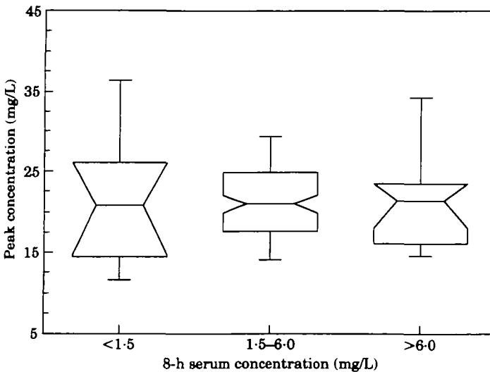
Figure 2. Box-plots displaying netilmicin peak concentrations for seven patients with 8-h serum concentrations of < 1.5 mg/L, 33 patients with 8-h concentrations of 1.5–6 mg/L and 11 patients with 8-h concentrations of > 6 mg/L.
