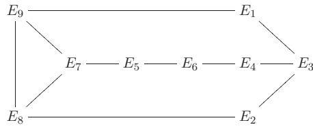
Fig. 3. Configuration of curves on \tilde{S} .
