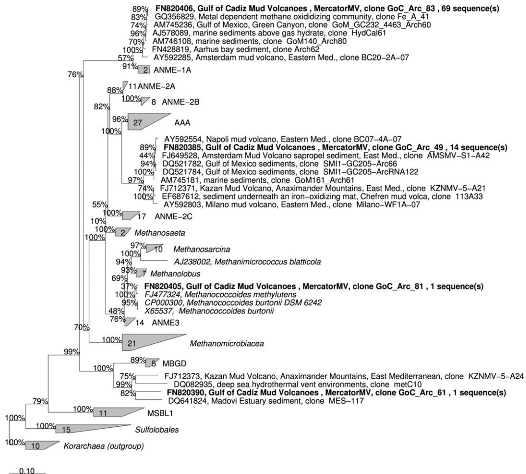
Fig. 4. Affiliation of Archaeal 16S rRNA gene sequences from Mercator MV Rim 1 (32–33 cmbsf). The phylogenetic tree was reconstructed based on a subset of 351 sequences using the maximum likelihood method (PhyML, Guindon et al. , 2009) filtering out positions according to base frequencies among Archaea (50% cutoff). Percentages indicate branch support as calculated by the aLRT bootstrapping method (Anisimova & Gascuel, 2006; Guindon et al. , 2009).
