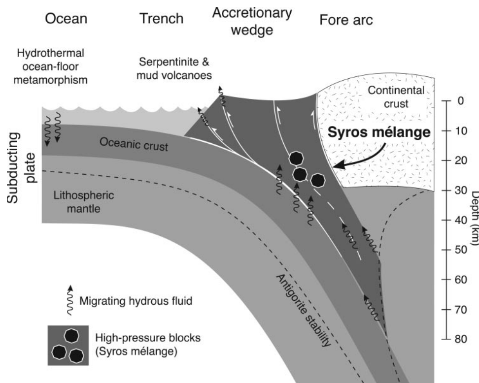
Fig. 8. Sketch of vertical cross-section through a subduction zone showing the exhumation channel located between the subducting slab on the left and the overlying plate on the right. High-pressure rocks, now exposed on the island of Syros, were rehydrated during their exhumation by aqueous fluids, probably released from the progressively subducted slab.
