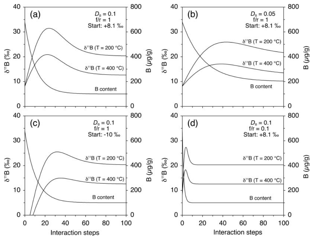
Fig. 11. Results of the model calculations on fluid–rock interaction with respect to \delta^{11}\text{B} and B concentrations of evolving fluids for two temperatures (200°C and 400°C). Diagrams (a)–(d) are calculated for different input parameters: (a) whole-rock–fluid partition coefficient D_B = 0.1 , fluid/rock mass ratio of each step ( f/r ) = 1, \delta^{11}\text{B} of initial fluid = +8.1‰; (b) D_B = 0.05 , f/r = 1 , \delta^{11}\text{B} = +8.1‰ ; (c) D_B = 0.1 , f/r = 1 , \delta^{11}\text{B} = -10.0‰ ; (d) D_B = 0.1 , f/r = 0.1 , \delta^{11}\text{B} = +8.1‰ .
