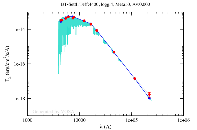
Figure 10. Spectral energy distribution and best-fitting model for J1407. Red points are the measured photometry with error bars. The dark blue points and line are the best fit to the photometric points, and the light blue is the model spectrum.
