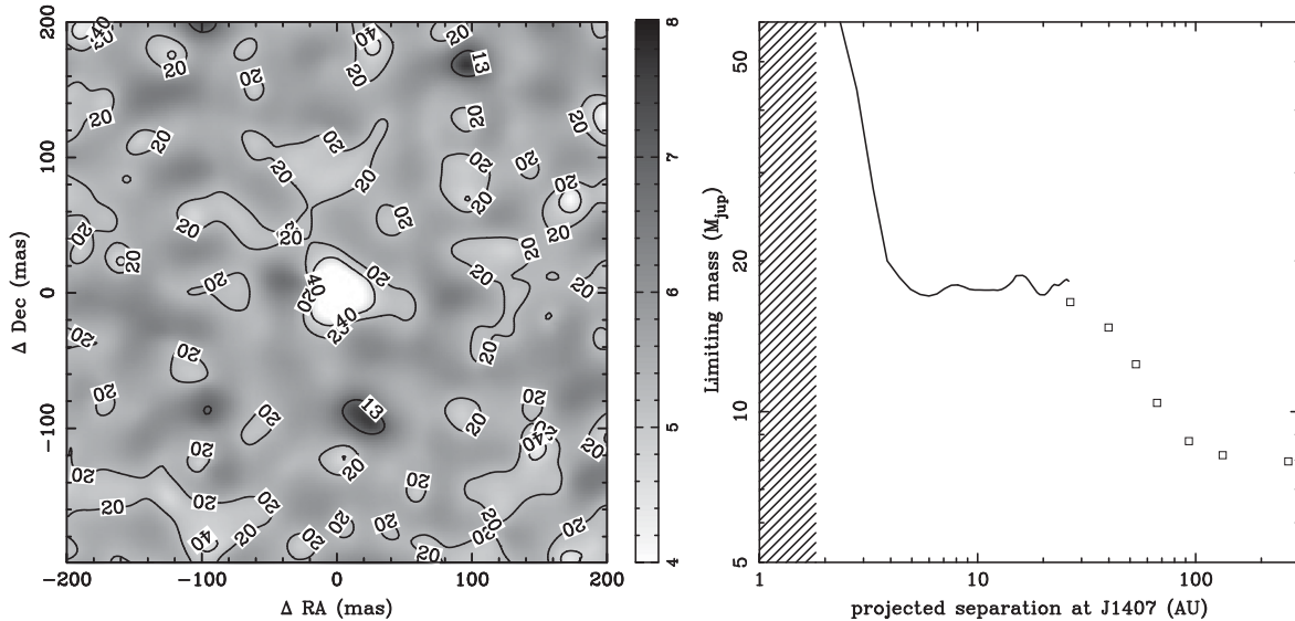
Figure 2. Sensitivity map of J1407 from SAM imaging at Keck. Left-hand panel: the star is at the centre of the image, the grey-scale and side bar indicate the sensitivity in delta K_s magnitudes for a 3\sigma point source detection. The contours indicate the associated upper mass limits in units of Jupiter masses ( M_{\text{Jup}} ) estimated from the K_s photometry and models from Allard et al. (2012a). North is up and east to the left. Right-hand panel: Azimuthally averaged sensitivity map. The hashed region indicates circular orbital periods of P < 850 d that are ruled out by Mamajek et al. (2012). The open squares are the sensitivity limits from direct imaging observations with Keck.
