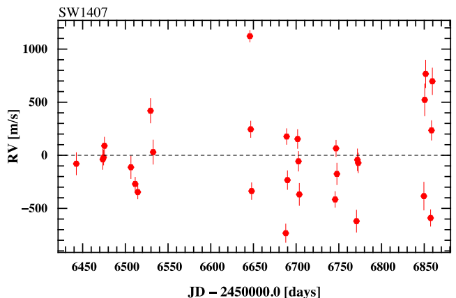
Figure 3. CORALIE measurements of the RV of J1407. The mean systemic velocity \gamma = 6.91 \pm 0.04 km s -1 has been subtracted off the data.
