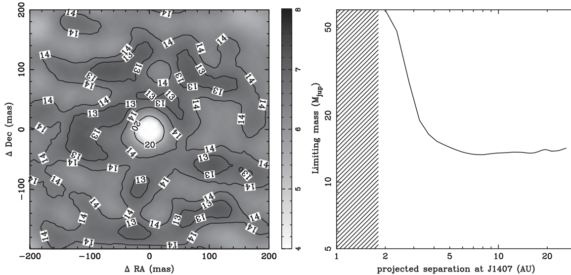
Figure 1. Sensitivity map of J1407 from SAM imaging at the VLT. Left-hand panel: the star is at the centre of the image, the grey-scale and side bar indicate the sensitivity in \Delta K_s magnitudes for a 3\sigma point source detection. The contours indicate the associated upper mass limits in units of Jupiter masses ( M_{\text{Jup}} ) estimated from the K_s photometry and models from Allard, Homeier & Freytag (2012a). North is up and east to the left. Right-hand panel: azimuthally averaged sensitivity map. The hashed region indicates circular orbital periods of P < 850 d that are ruled out by Mamajek et al. (2012).
