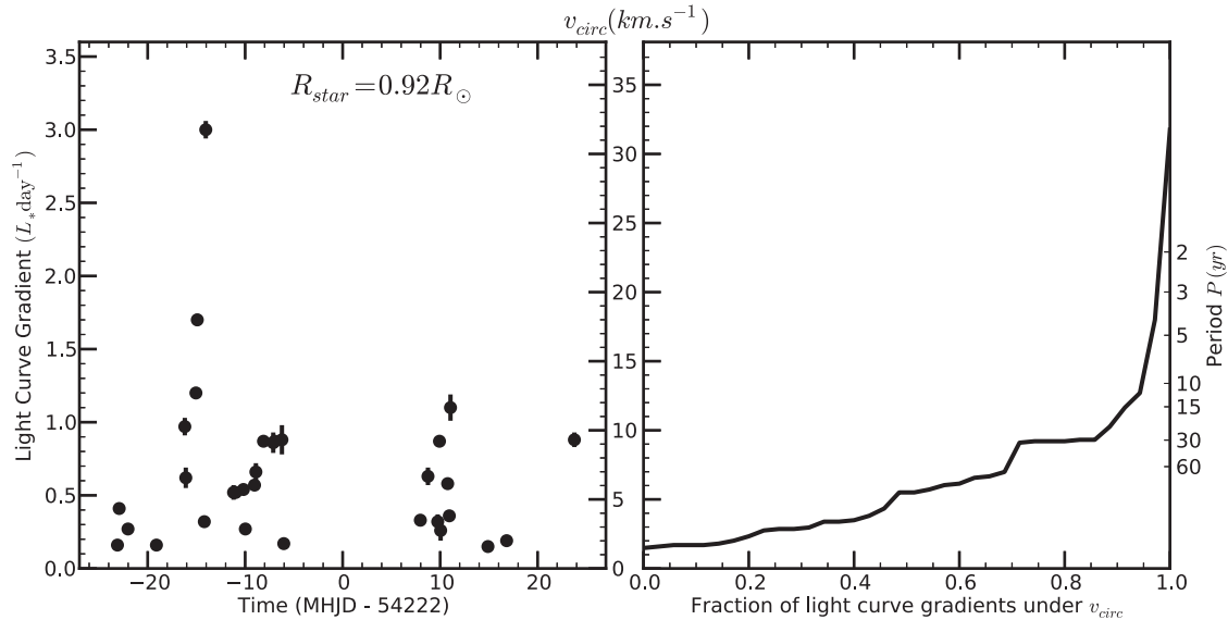
Figure 11. Gradients of the J1407 light curve as a function of time. The gradients are taken from van Werkhoven et al. (2014) and a stellar radius R_* = 0.92 R_{\odot} adopted. The right-hand scale shows the transverse velocity required to produce that gradient.
