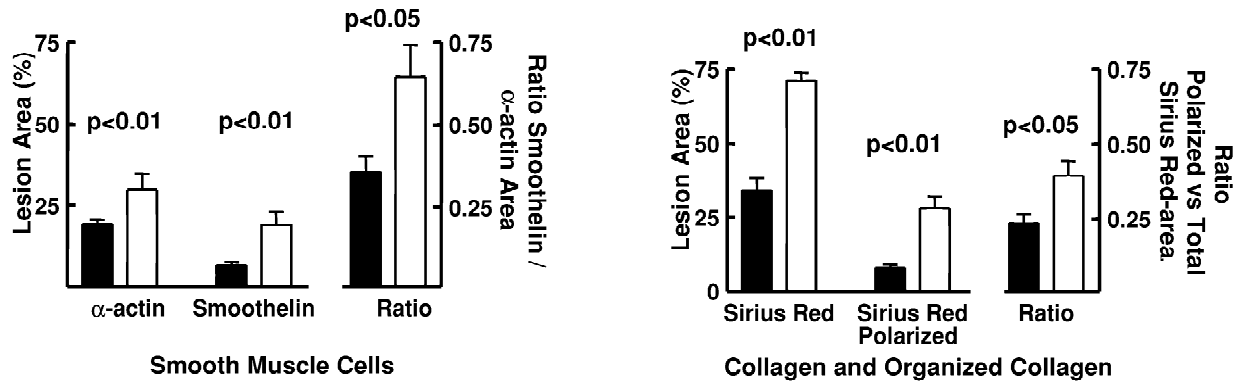
Fig. 3. Mean \alpha -SM actin and smoothelin areas in advanced lesions from hypercholesterolemic pigs (■) and from pigs after dietary cholesterol withdrawal (□). Lesions from hypercholesterolemic pigs contained less smooth muscle cells that were less differentiated as indicated by the lower smoothelin-to- \alpha -SM actin ratio. Lesions after cholesterol withdrawal contained more collagen that was more organized.
