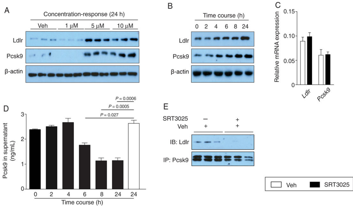
Figure 4 SRT3025 increases Ldlr expression in AML12 hepatocytes and decreases Pcsk9 in the supernatant. Western blots of Ldlr, Pcsk9, and β-actin in cultured AML12 cells (A) treated with SRT3025 at indicated concentrations for 24 h and (B) incubated with 10 μM SRT3025 for the times indicated. (C) Relative mRNA expression levels of Ldlr and Pcsk9 in AML12 cells after incubation with 10 μM SRT3025 for 24 h. (D) Pcsk9 protein levels in the supernatant of AML12 cells incubated with 10 μM SRT3025 for the times indicated. (E) Pcsk9 immunoprecipitated from AML12 cells incubated with vehicle (Veh, DMSO) or 10 μM SRT3025, and blotted for Ldlr and Pcsk9. Pcsk9, proprotein convertase subtilisin/kexin type 9.
