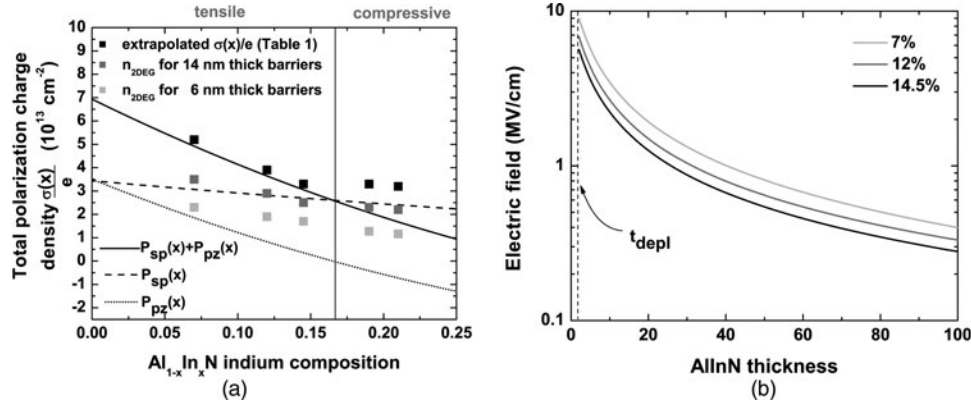
Fig. 6. (a) Lines correspond to spontaneous (—) and piezoelectric (···) polarization charges and the sum of both (—) at RT for an AlInN random alloy, 2DEG densities for 6 nm thick (gray squares), 14 nm thick (dark gray squares) AlInN barriers, and the extrapolated total bound. (b) Electric field across the AlInN barrier for 7, 12, and 14.5% indium calculated from equation (2) using the parameters from Table 1.
