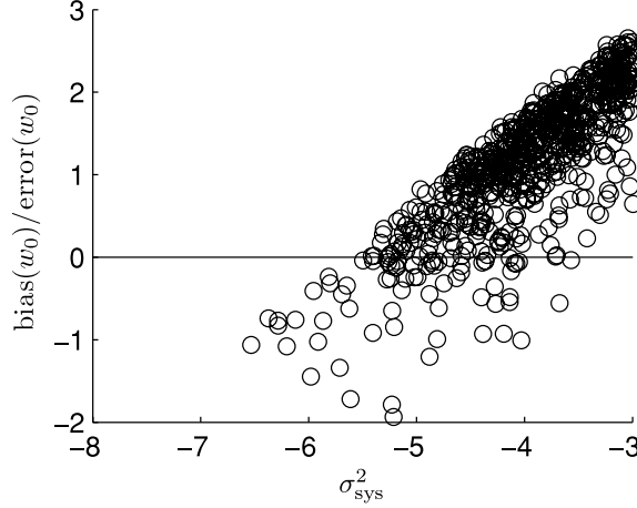
Figure B1. Monte Carlo realizations of submitted shear power spectrum where \sigma_{\text{sys}}^2 is the denominator in equation (B1), and the calculated bias in dark energy parameter with respect to its error.
