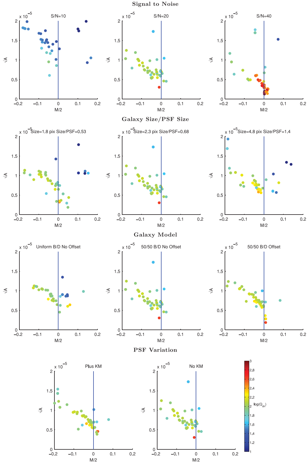
Figure 4. In each panel, we show the metrics, \mathcal{M} , \mathcal{A} and Q_{\text{dn}} , for each of the parameter variations between sets, for each submission; the colour scale labels the logarithm of Q_{\text{dn}} as shown in the lower right-hand panel. The first row shows the S/N variation, the second row shows the galaxy size variation, the third row shows the galaxy model variation (the galaxy models are: uniform bulge-to-disc ratios where each galaxy has a bulge-to-disc ratio randomly sampled from the bulge-to-disc ratio range [0.3, 0.95] with no offset (Uniform B/D No Offset), a 50 per cent bulge-to-disc ratio = 0.5 with no offset (50/50 B/D No Offset) and a 50 per cent bulge-to-disc ratio = 0.5 with a bulge-to-disc centroid offset (50/50 B/D Offset), and the fourth row shows PSF variation with and without Kolmogorov (KM) PSF variation.
