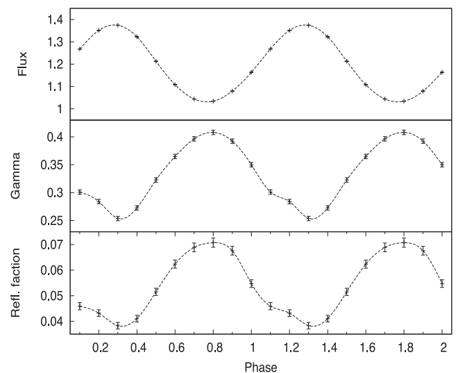
Figure 14. Best-fitting parameters 1\sigma errors for the 10 phase-resolved spectra. From top to bottom: RELXILL 0.5–10 keV unabsorbed flux in units of 10^{-8} erg cm^{-2} s^{-1} , photon index and reflection fraction.
