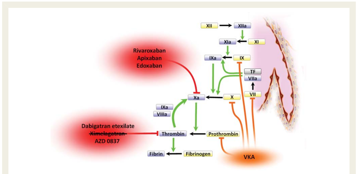
Figure 1 Point of action of novel oral anticoagulants in the coagulation cascade.
