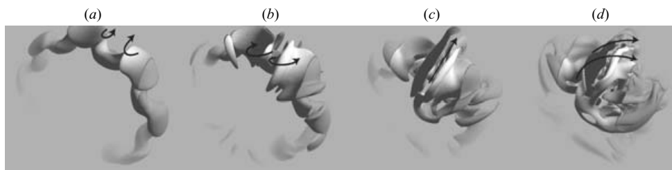
FIGURE 4. Emergence of the secondary vortical structures ( a–d ): the Tsai–Widnall, or shortwavelength instability leads to the formation of a dipole which is stretched and convected in the streamwise direction.
