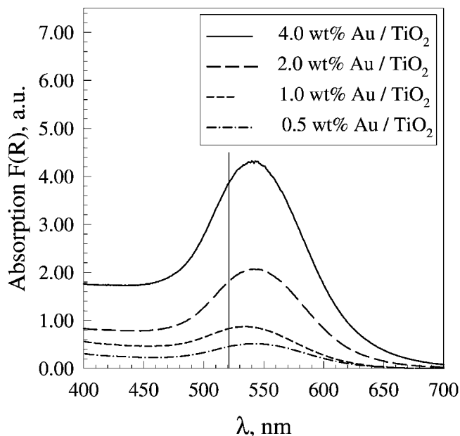
FIG. 9. UV-vis spectra of 0.5, 1, 2, and 4 wt% Au on titania. Different amounts of gold loadings do not change the peak location of the plasmon band, indicating that the gold crystallites are smaller than 20 nm. The peak position of the spectra (540 nm) is red shifted compared to the pure gold plasmon peak (vertical line), indicating a weak interaction between the gold and the support.
