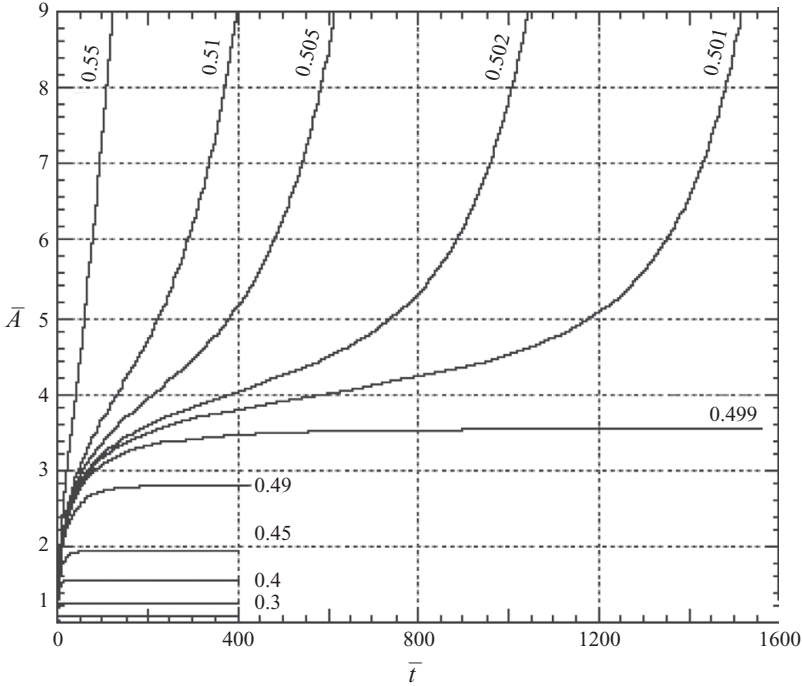
FIGURE 15. Theoretically predicted evolution of the mean cross-section as a function of non-dimensional time for various non-dimensional inflow rates. For non-dimensional inflow rates less than 1/2, the membrane reaches a stationary plateau, whereas for inflow rates larger than 1/2, the maximum cross-section diverges in finite time.
