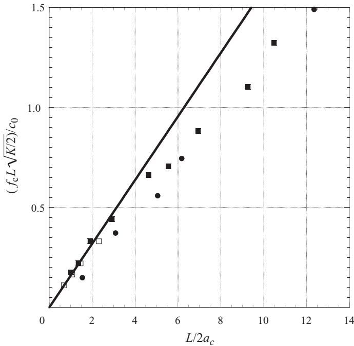
FIGURE 16. Non-dimensional critical frequency at the onset of an aneurysm \bar{f}_c = ((L\sqrt{K/2})/c_0)f_c as a function of L/2\bar{a}_c , half the inverse of the non-dimensional critical amplitude \bar{a}_c = a_c/L for the aneurysms reported in figure 14. The predicted linear dependence with slope 1/2\pi is shown by the solid line.
