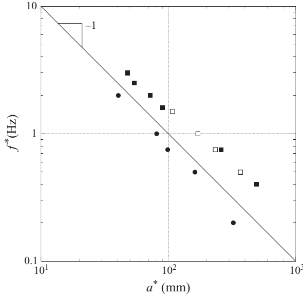
FIGURE 14. Amplitude and frequency threshold above which a bulge grows without bounds for several hydraulic outlet resistances and lengths. (●) K = 40 , L = 1 m; (■) K = 14 , L = 1 m; (□) K = 14 , L = 0.5 m.
