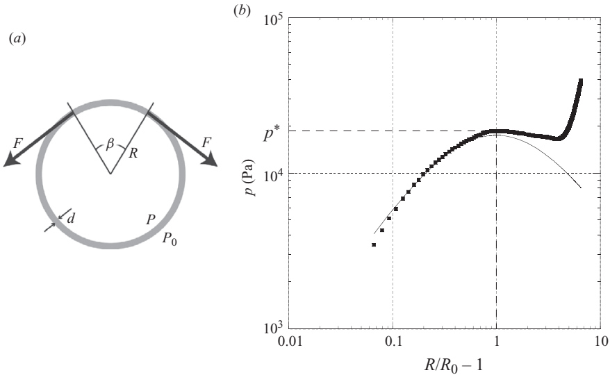
FIGURE 4. A pressure law for the cylindrical membrane: (a) scheme for the equilibrium, (b) experimental evolution of the transmural pressure p with the relative deformation R/R_0 - 1 (■). The solid line corresponds to the theoretical curve (2.2).
