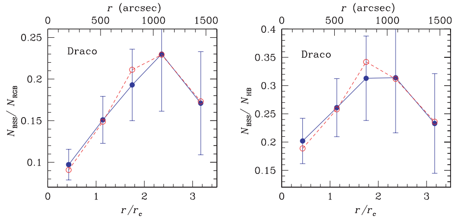
Figure 6. Relative frequency of BSSs normalized to RGB (left-hand panel) and HB stars (right-hand panel) in Draco. The filled circles connected by the solid line are the measurements (the same as in Fig. 3). The open circles connected by the dashed line are the fiducial model (run A1).
