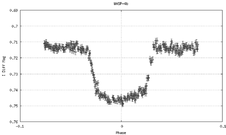
Figure 1. Ligth Curve of WASP-4b.
