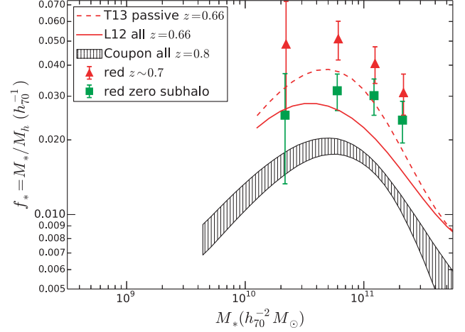
Figure D1. SHMR for CFHTLenS red galaxies at z \sim 0.7 comparing the estimated halo mass including the default assumption that satellites have partially stripped subhaloes (red triangles) and setting their subhalo contribution to zero (green squares). The latter assumption is adopted in the GGL analysis of T13, L12 and Coupon et al., whose fits are shown by the dashed red line (passive galaxies), solid red line (all galaxies) and hatched area (all galaxies), respectively.
