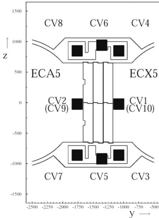
Figure 3. Horizontal section through the main shield indicating the positions of the CV.
