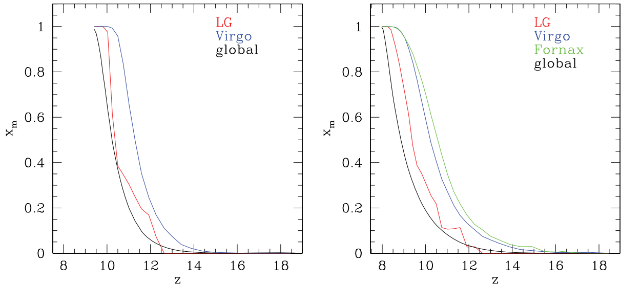
Figure 4. Mass-weighted mean ionized fractions, x_m , for the Local Group, nearby clusters and global mean (as indicated by colour) versus redshift for Model 1 (left; left to right: global, LG, Virgo) and Model 2 (right; left to right: global, LG, Virgo, Fornax).
