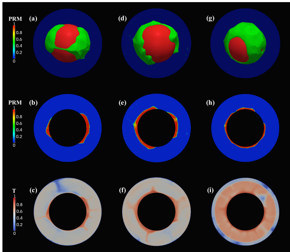
Figure 15. Snapshot of cases with B = 0.30 , X_{\text{vol}} = 3.5 per cent, \Delta\eta_T = 10^9 , t = 0.0117 (4.5 Gyr) and (from left to right): 660 km Clapeyron slope ( \Gamma_{660} = 0, -2.5, -5 MPa \text{K}^{-1} ). Top row: isosurface of the composition with contour level C = 0.5 . Middle row: polar slice of the composition. Bottom row: polar slice of the temperature.
