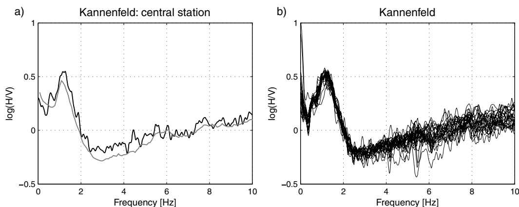
Figure 14. (a) H/V spectral ratios obtained for the central station for array at Kannenfeld. The black line is the result of the classical polarization analysis in the frequency domain. It was corrected for SH waves using the assumption of equal amplitude of SH and P-SV waves on the horizontal components. The grey line was obtained with the method based on the frequency-time analysis. (b) Comparison of the H/V spectral ratios of all stations in the array using the classical polarization analysis.
