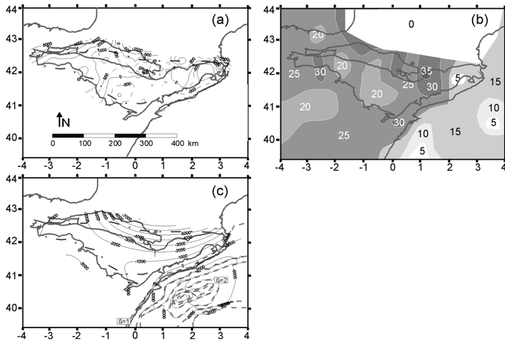
Figure 10. Modelling results for a broken plate with variable T_e values and a line load of -2 \times 10^{12} \text{ N m}^{-1} at the northern edge, including the effect of the Valencia Trough rifting (stretching factors modified from Collier et al. 1994; Ayala et al. 1996 and Watts & Torné 1992). (a) Deviation plot (see Fig. 7 for explanation). (b) T_e map derived from the heat flow map of Fernández et al. (1998) by a simple linear inverse relation ( T_e \propto -\text{heat flow} ). (c) Contour lines of calculated deflection. In this case \beta = \beta_m = \beta_c . Other figure conventions as in Fig. 8.
