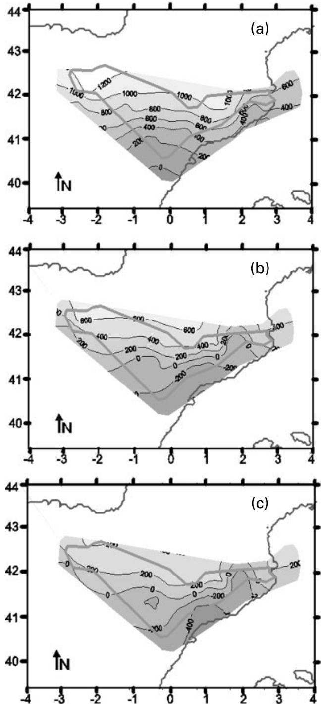
Figure 4. Contour maps of subsidence values derived from well data (Lanaja 1987). The contour interval is 200 m. The residual surface (RS) is defined as follows: residual\ surface = air-loaded\ subsidence - topography . Zero RS values imply that the sediment infill (topography-corrected) is locally isostatically compensated, positive RS values imply that an extra force is pulling the plate downwards, and negative values imply that a force is pushing it upwards. (a) Air-loaded (i.e. resulting from the back-stripping, without topographic correction); (b) residual with compaction; (c) residual without compaction (constant sediment density).
