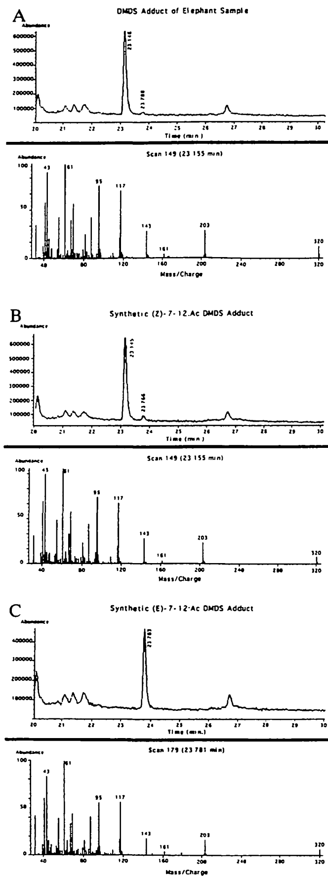
Figure 6 GC-MS of elephant pheromone (A), compared with synthetic Z -7-12:Ac DMDS adduct (B), and synthetic E -7-12:Ac DMDS adduct (C). A comparison of retention times with those of synthetic standards showed that the larger adduct peak (97%) at 23.15 min was the Z isomer, and the smaller one at 23.78 min was the E isomer. The mass spectra of the DMDS adducts of elephant-derived ( Z )-7-dodecen-1-yl acetate (A, bottom) were identical to those produced by synthetic Z -7-12:Ac (B, bottom) and E -7-12:Ac (C, bottom). A comparison of retention times of the synthetic standards with those of the adducts showed that the larger adduct peak at 23.15 min was the Z isomer (B) and the smaller one at 23.78 min was the E isomer (C). The initial assay of the elephant pheromone was 97% of Z -7-12:Ac and 3% of E -7-12:Ac.
