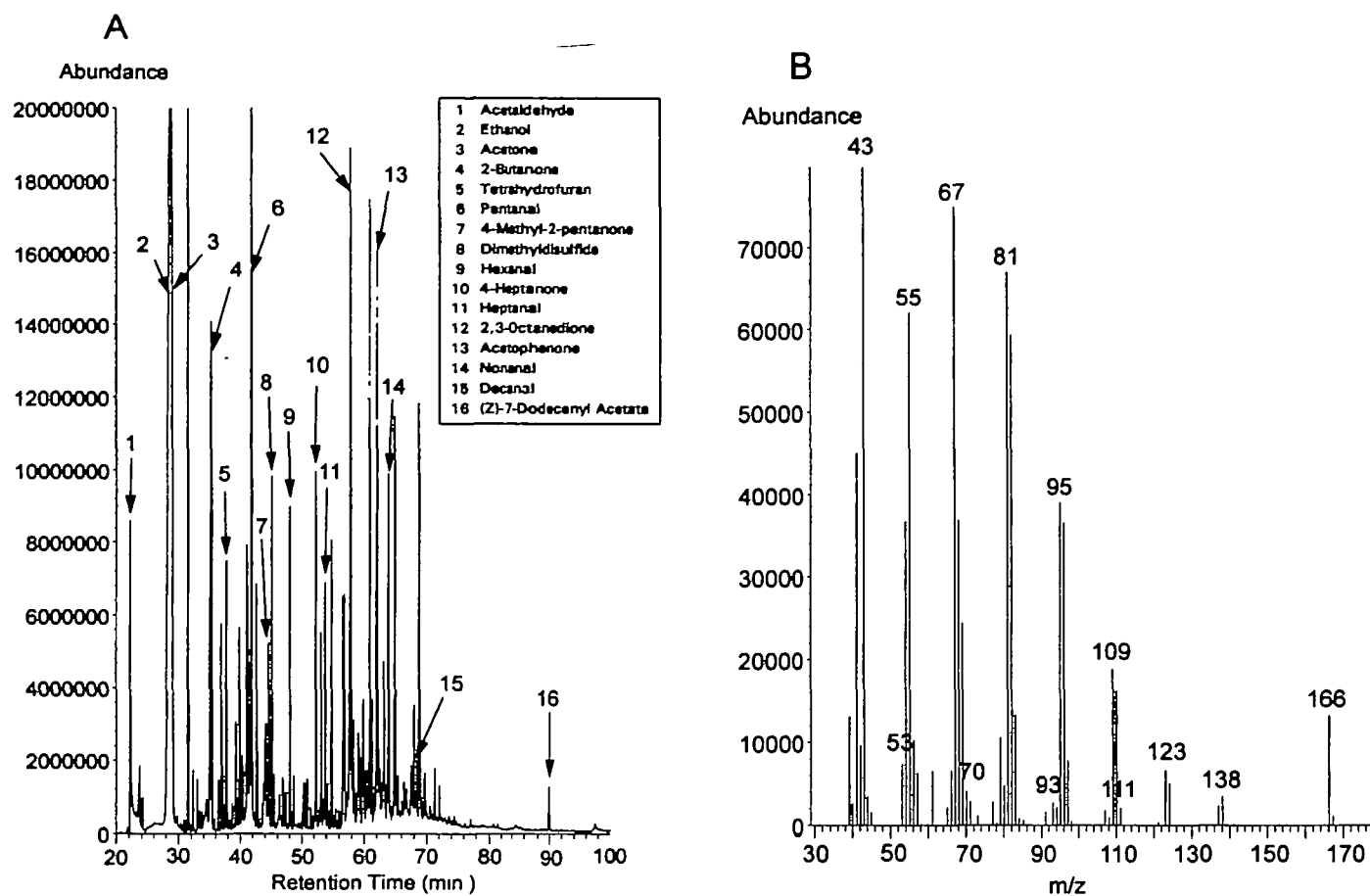
Figure 7 (A) GC-MS total ion chromatogram of the headspace of female pre-ovulatory urine, assessed bioactive by responses of male Asian elephants. Fifteen relatively common volatiles in female urinary headspace are indicated, these ranged from ~50 to 500 ppbv Z7-12:Ac (peak 16) was detected at a late retention time (B) GC-MS spectrum of the fragment ion of the late-eluting Z7-12:Ac
