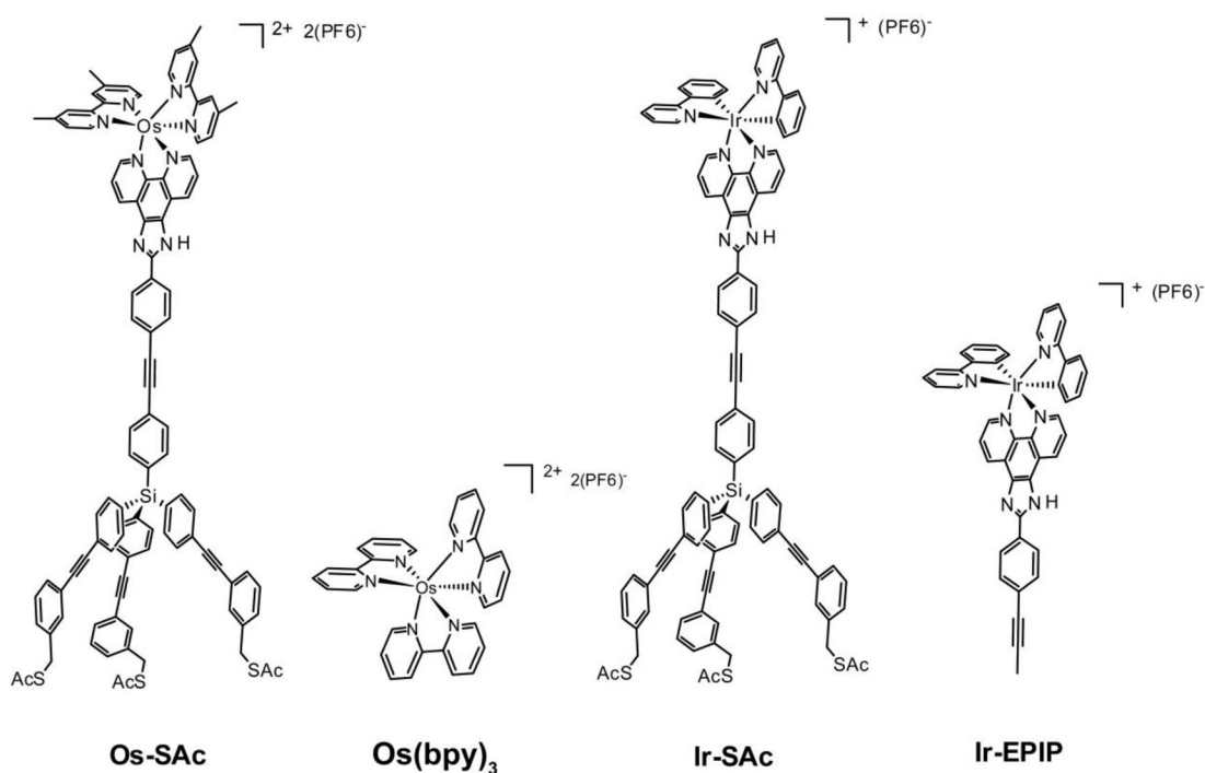
Scheme 1 Schematic formulas of the Ir and Os tripodal complex investigated along with their respective reference compounds. The molecules will be named with the abbreviation shown under the structure. To evidence the tripodal structure and the possible geometry adopted on the surface the anchoring groups are drawn all in the same direction.
