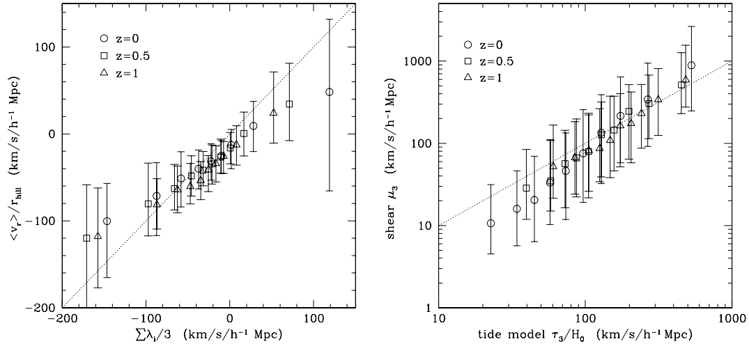
Figure 3. Comparisons between the flux on to haloes from particle velocities and in the CSA model, and between the tides due to the tidally dominant neighbour halo and measured shear in the CSA. Left-hand panel: the flow through the Hill sphere \sum_i \lambda_i/3 from the linear fit to the flow against median \langle v_r \rangle / r_{\text{Hill}} measured directly from the simulation. Results are shown for haloes with r_{\text{Hill}} \leq 4r_{\text{vir}} , the region used for determining the \lambda_i . Right-hand panel: median eigenvalue of the shear tensor \mu_3 measured from the flow as a function of the tidal force due to the tidally dominant neighbour halo \tau_3 = 2GM/R^3 . Error bars show the 16th and 84th percentiles in each bin. Bins are chosen to include equal numbers of data points. The dotted lines indicate x = y . Data are given for the progenitors of haloes with masses between 2 and 4 \times 10^{10} h^{-1} M_\odot .
