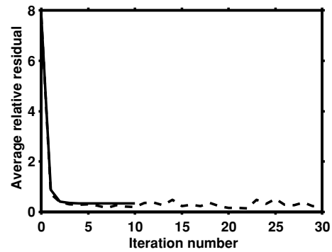
Figure 6. Average relative residuals ( ARR = \frac{100}{N} \sum_{i=1}^N |t_i^{\text{true}} - t_i^{\text{pre}}| / t_i^{\text{true}} ) as functions of the iteration number for conventional tomography (solid line) and discrete tomography (dashed line) applied to traveltime data computed for the velocity model in Fig. 2(b). The average relative residual at ‘iteration 0’ was calculated for the input homogeneous model.
