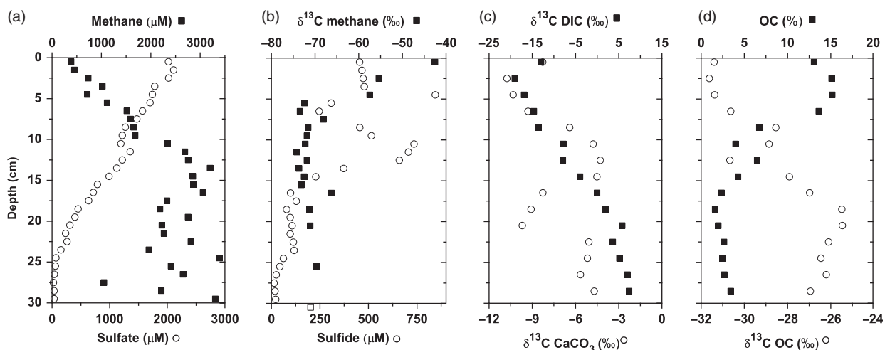
Fig. 1. Geochemical gradients in Lake Cadagno sediment core. (a) Methane and sulfate concentrations in \mu\text{M} . (b) Sulfide concentrations in \mu\text{M} and \delta^{13}\text{C} of methane (in ‰ vs. Vienna Pee Dee Belemnite, VPDB). (c) Carbon isotope values (in ‰ vs. VPDB) of dissolved inorganic carbon (DIC) and carbonate. (d) Organic carbon concentrations (% of dry weight) and carbon isotopic composition (in ‰ vs. VPDB).
