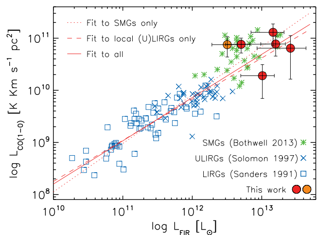
Figure 7. Lens-corrected CO luminosity versus FIR luminosity ( L'_{\text{CO}}-L_{\text{FIR}} ) for our sample, in red circles, and in light red if we adopt the alternative CO solution for HLS J045518.0+070103. For galaxies with more than one detected transition we have plotted the mean L'_{\text{CO}} . For comparison, other SMGs are plotted (Bothwell et al. 2013) along with local LIRGs (Sanders et al. 1991) and ULIRGs (Solomon et al. 1997). Best-fitting slopes derived by Bothwell et al. (2013) to SMGs, local (U)LIRGs, and all three combined samples are overplotted. They have slopes of 0.93 \pm 0.14 , 0.79 \pm 0.08 , and 0.83 \pm 0.09 , respectively.
