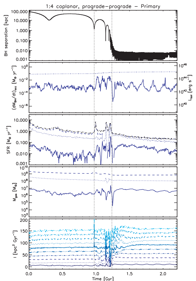
Figure 2. Temporal evolution of the 1:4 coplanar, prograde–prograde merger – main quantities of and around the primary BH. Same as Fig. 1. BH accretion rate, non-total SFR and gas mass are shown in blue. In the fifth panel, the colour of the specific-angular-momentum of each gas shell varies from dark to light blue as the radius of the shell increases.
