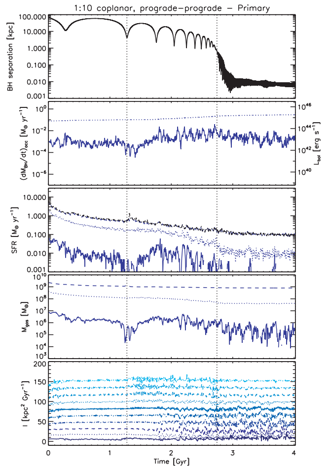
Figure A4. Temporal evolution of the 1:10 coplanar, prograde-prograde merger – main quantities of and around the primary BH. Same as Fig. 2.
