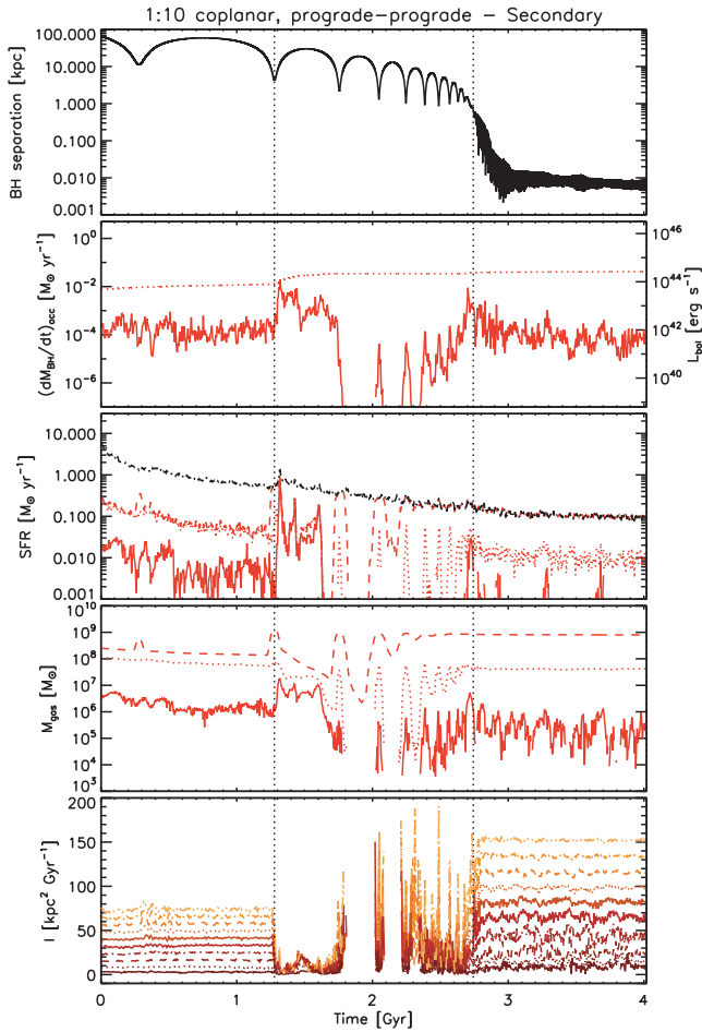
Figure A3. Temporal evolution of the 1:10 coplanar, prograde-prograde merger – main quantities of and around the secondary BH. Same as Fig. 1.
