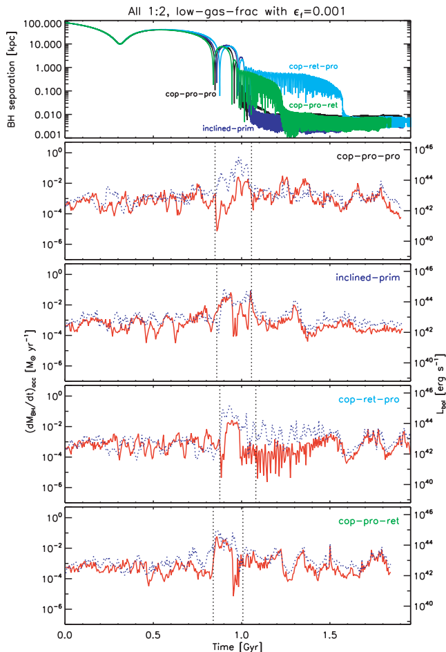
Figure 13. BH accretion rates for all 1:2 mergers with low gas fraction and \epsilon_f = 0.001 . In panels 2–5, the vertical, dotted, black lines show the separation between the stochastic, the merger, and the remnant stages. First panel: separation between the two BHs, for the prograde–prograde (black), inclined–primary (blue), retrograde–prograde (cyan), and prograde–retrograde (green) merger. Second panel: BH accretion rate for the primary (dotted, blue) and secondary (solid, red) BH of the prograde–prograde merger. Third panel: same as the second panel, but for the inclined–primary merger. Fourth panel: same as the second panel, but for the retrograde–prograde merger. Fifth panel: same as the second panel, but for the prograde–retrograde merger.
