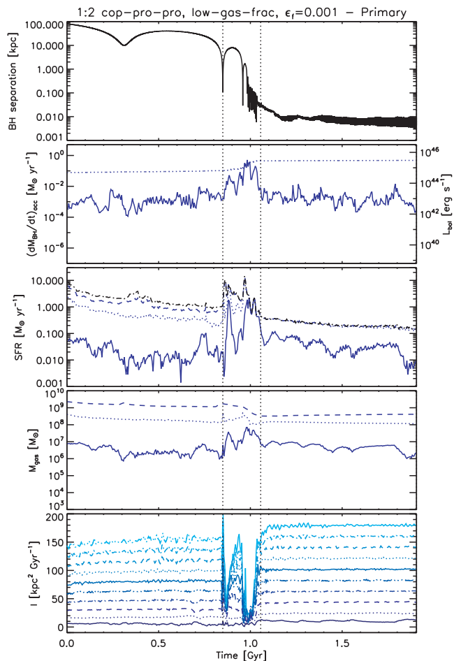
Figure A2. Temporal evolution of the 1:2 coplanar, prograde–prograde merger with low gas fraction and \epsilon_f = 0.001 – main quantities of and around the primary BH. Same as Fig. 2.
