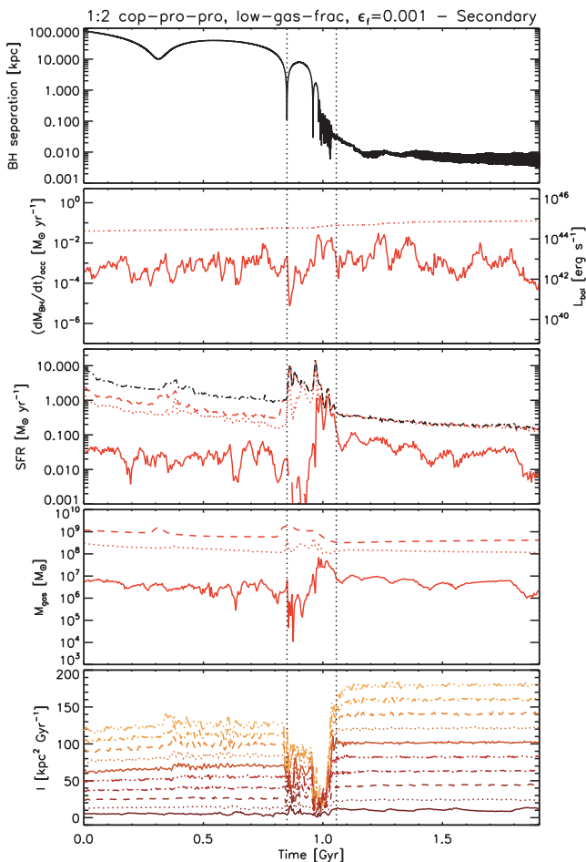
Figure A1. Temporal evolution of the 1:2 coplanar, prograde–prograde merger with low gas fraction and \epsilon_f = 0.001 – main quantities of and around the secondary BH. Same as Fig. 1.
