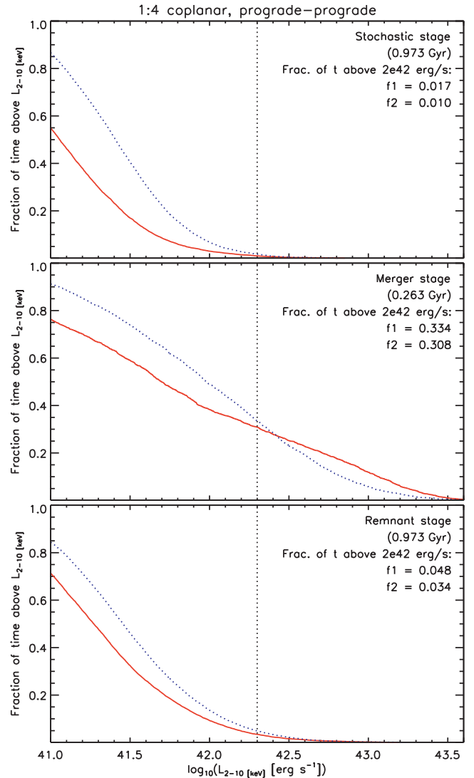
Figure 5. Fractional cumulative time above a given luminosity, for the primary ( f1 ) and secondary ( f2 ) BH, in the 1:4 coplanar, prograde–prograde merger. For each stage of the merger, we show the cumulative time, divided by the time-length of the stage, for which a BH accretes above a given level, as a function of the inferred hard-X-ray luminosity. The vertical, dotted, black line shows the typical AGN-activity threshold ( L_{2-10\text{keV}} \simeq 2 \times 10^{42} \text{ erg s}^{-1} ). Top panel: fractional cumulative time for the stochastic stage, for the primary (dotted, blue) and for the secondary (solid, red) BH. Middle panel: same as the top panel, but for the merger stage. Bottom panel: same as the top panel, but for the remnant stage.
