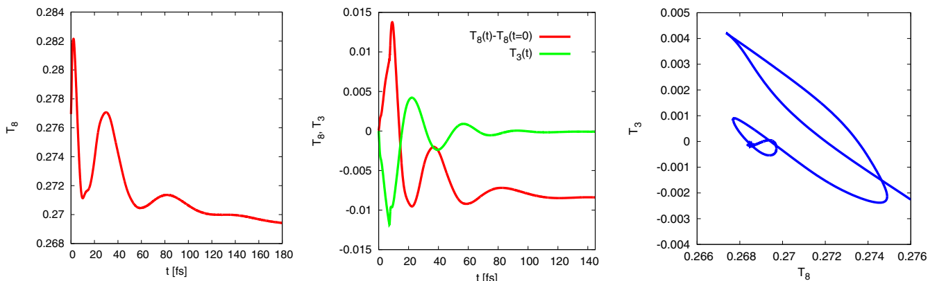
FIG. 5. Excitation of amplitude and phase modes in the model with \gamma = 1 . The left panel shows \mathcal{T}_8 after a 20% reduction in all hoppings at t = 0 . In the middle panel, the hopping quench is delayed by \Delta t = 7.3 fs for orbitals 1 and 3, which allows one to also excite oscillations in \mathcal{T}_3 . The right panel shows the evolution in the \mathcal{T}_8 - \mathcal{T}_3 plane after this double-quench.
