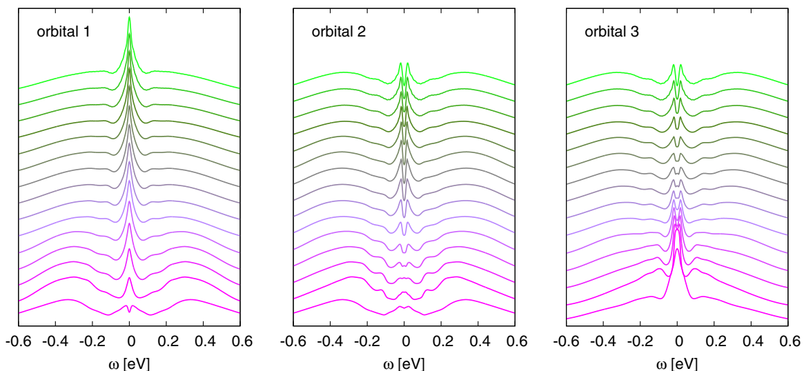
FIG. 3. Switching from T_z = (I, I, M) to T_x = (M, I, I) . From bottom to top: Local spectral functions for times t = 0, 14.5, 29, \dots, 203 fs. The spectra have been obtained by Fourier transformation on the time interval from t to t_{\max} = 280 fs [22].
