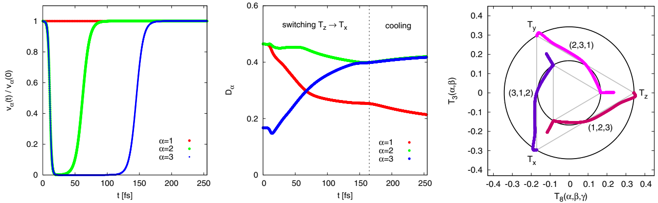
FIG. 2. Switching between T_8 > 0 states by suppression of hopping ( U = 1 eV, J = -0.25 eV, T = 33 K). The order parameter can be defined in terms of the linear combinations T_8(\alpha, \beta, \gamma) = (D_\alpha + D_\beta - 2D_\gamma)/\sqrt{3} and T_3(\alpha, \beta) = D_\alpha - D_\beta . The initial state is T_z = (I, I, M) , with order parameter T_8(1, 2, 3) > 0 , T_3(1, 2) = 0 , and the state after the switching is T_x = (M, I, I) . The left panel shows the time evolution of the hopping parameters for the three orbitals, the middle panel the time evolution of the double occupancy, and the right panel the (clockwise) rotation of the order parameter in the T_8 - T_3 plane.
