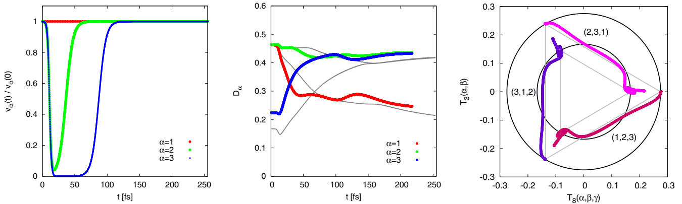
FIG. 4. Switching between \mathcal{T}_8 > 0 states in the model with rotationally invariant interaction ( \gamma = 1 ). The left panel shows the switching protocol and the middle panel the time evolution of the double occupancy with gray lines, taken from Fig. 2 ( \gamma = 0 ), as a reference. The right panel shows the (clockwise) rotation of the order parameter in the \mathcal{T}_8 - \mathcal{T}_3 plane.
