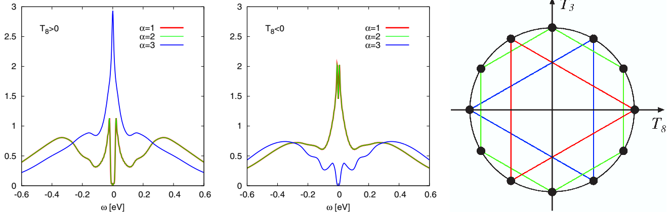
FIG. 1. Orbital-dependent spectral functions A_\alpha(\omega) = -\frac{1}{\pi}\text{Im}G_\alpha(\omega) for the equilibrium SOSM state corresponding to T_8 > 0 , T_3 = 0 (left panel) and T_8 < 0 , T_3 = 0 (middle panel). The spectra have been obtained for U = 1 eV, J = -0.25 eV, T = 33 K using the NCA impurity solver. Right panel: Equivalent SOSM states connected by permutations of the orbitals. The stable solutions are the three states equivalent to T_8 > 0 , T_3 = 0 (red triangle).
