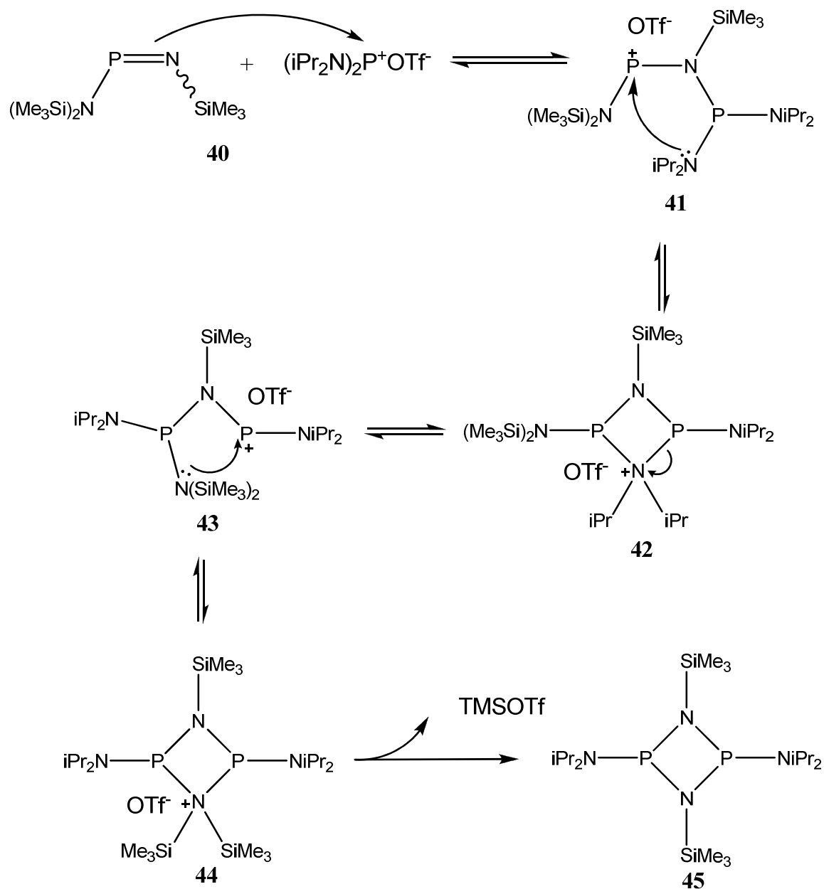
Scheme 30: Modified scheme for the mechanism of formation of a diazadiphosphetidine from the reaction of (\text{iPr}_2\text{N})_2\text{P}^+\text{OTf}^- with an iminophosphorane taken from Sanchez et al. 51
