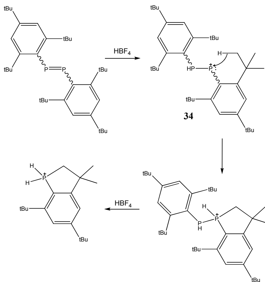
Scheme 25: A reactive phosphenium ion intermediate
