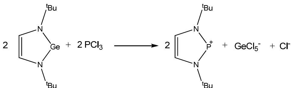
Scheme 13: Synthesis of a cyclic phosphenium ion from a germylene
