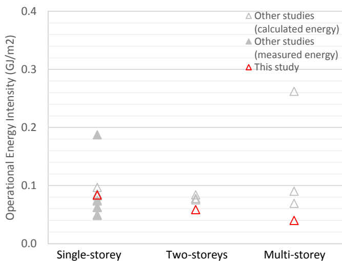
Figure 6 Comparison of operational energy results (reference case) with other studies in literature. Results for composite climate.
