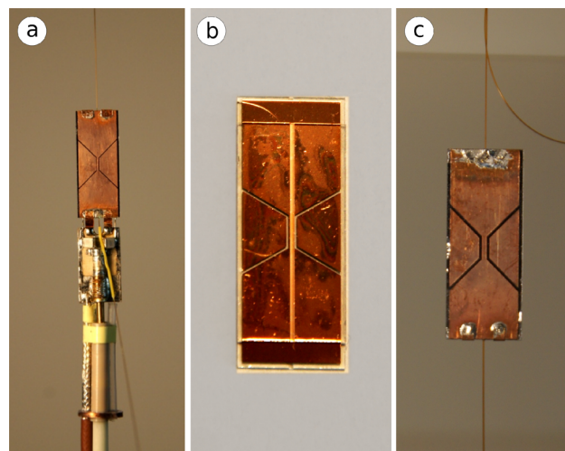
Figure 1. NMR stripline chips used in this study: chip a, chip b, and chip c.
