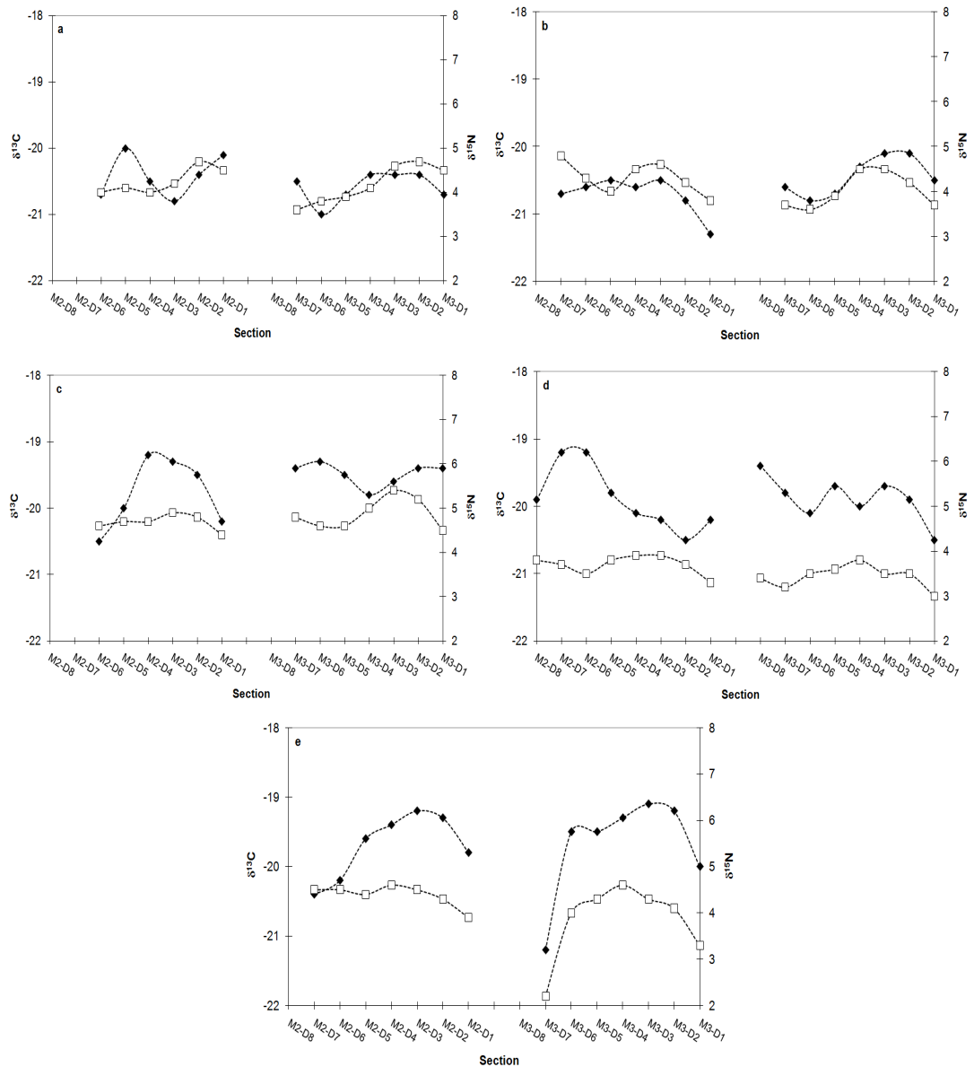
Figure 7.4 \delta^{13}\text{C} and \delta^{15}\text{N} values from collagen from sequentially sampled dentine from individuals of the Western Arctic caribou herd, Alaska. (a= WACH-2.210, b= WACH-2000, c= WACH-0.120, d= WACH-2.230, e= WACH-153.180). Solid diamonds = carbon, open squares = nitrogen.
