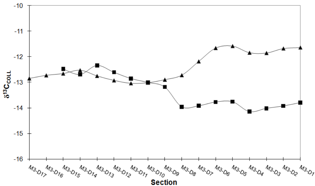
Figure 7.28 Carbon isotope ( \delta^{13}\text{C} ) values of collagen from the sequentially sampled dentine from Wichita Mountains bison herd.
