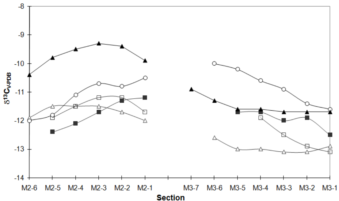
Figure 7.3 Plot of all carbon isotope data ( \delta^{13}\text{C}_{\text{V-PDB}} ) from intra-tooth sections from M2 and M3 enamel of each of the five animals analysed from the Western Arctic caribou herd, Alaska.
