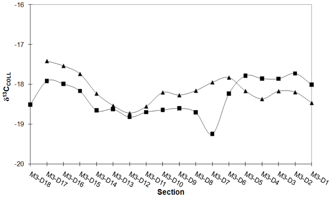
Figure 7.23 Carbon isotope values ( \delta^{13}\text{C} ) values from collagen from sequentially sampled dentine from individuals of the Wind Cave National Park bison.
