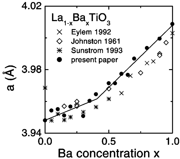
FIG. 1. Lattice parameter a of \text{La}_{1-x}\text{Ba}_x\text{TiO}_3 vs barium concentration x . The solid circles ( \bullet ) are the values reported in the present paper; the other symbols represent values taken from literature ( \times , Ref. 12, \diamond , Ref. 13, * Ref. 9). The solid line is drawn to guide the eye.
