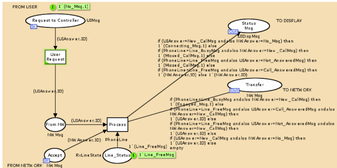
Fig. D.7 'Handset Controller common component subnet'
