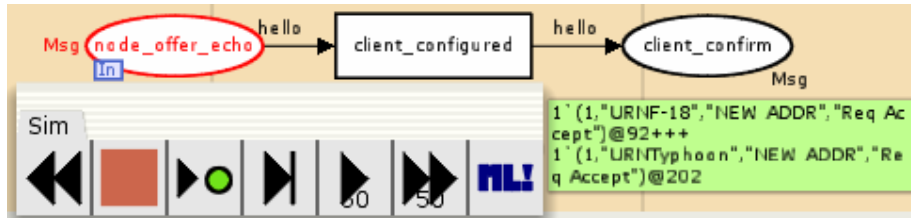
Fig. 6.10 'Capture of model time for client_configured transition'
