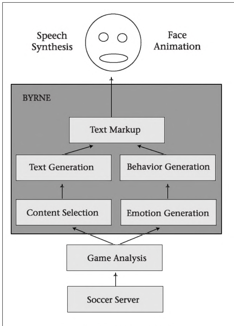
Figure 3. The BYRNE System Architecture.
