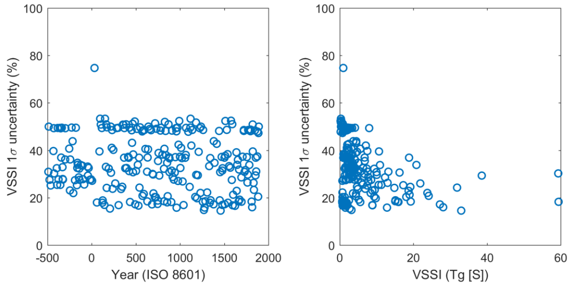
Figure S6: Estimated 1sigma uncertainties in eVol2k VSSI data set plotted as a function of (left) year, and (right) VSSI.
