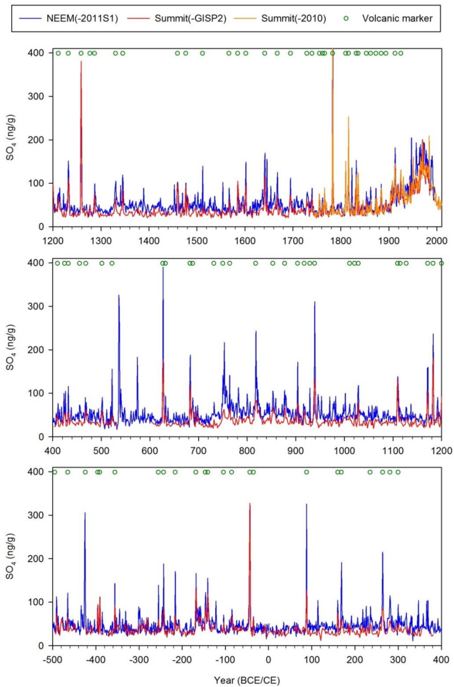
Figure S2: As Fig. S1 for the three time periods (from top): 1200-2010 CE, 400-1200 CE and 500 BCE-400 CE.
