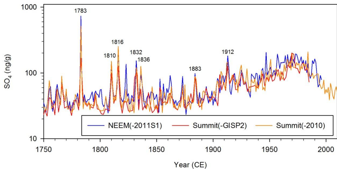
Figure S3: As Fig. S1 but for the time period 1750-2010 CE with concentrations on a logarithmic scale and the seven largest volcanic sulphate deposition events denoted.
