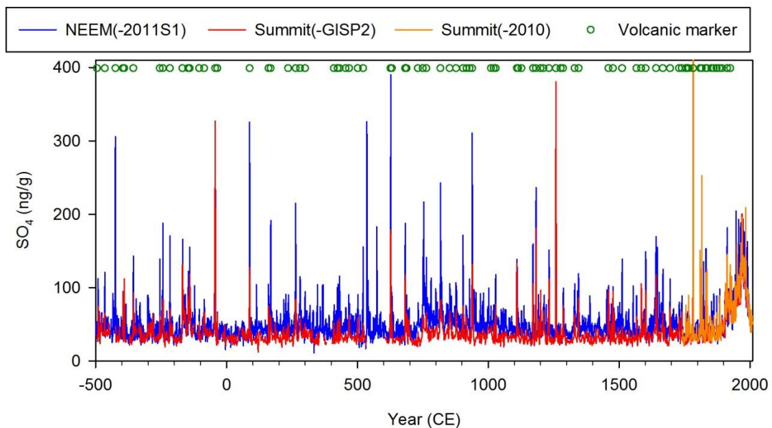
Figure S1: GISP2 SO 4 record from Greenland Summit (Zielinski et al., 1995, 1996) synchronized to the NEEM(-2011-S1) ice core on the NS1-2011 timescale (Sigl et al., 2013, 2015) using 85 volcanic marker horizons (green circles). The GISP2 record has been updated with the Summit(-2010) firn core drilled at the same site in 2010 (Maselli et al., 2017).
