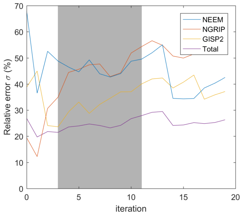
Figure S5: Percent errors estimated for each of the three Greenland ice core sulphate records using the method described in Appendix A. The first iteration of the analysis used the 48 strongest sulphate signals present in all three cores; each subsequent iteration removed from consideration the event with the largest average value across the three cores. The values of estimated error for each ice core record, and the estimated total error of the mean, are plotted as a function of iteration number (or, equivalently, number of largest values removed from the analysis). The grey shaded region denotes the range of relative stability in the error estimates, over which the values were averaged to produce best estimates of the random error in each ice core record.
