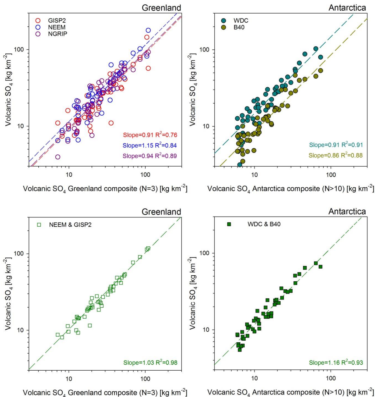
Figure S4: Upper panels: Scatterplot between volcanic sulphate flux for individual ice cores and ice-core composite records for Greenland (left) and Antarctica (right); lower panels: as above for the pairs of ice cores used for reconstruction prior to the Common Era. Included in the analysis are all events common to all three ice cores from Greenland and all events for Antarctica with sampling coverage of the composite >10 ice cores.
