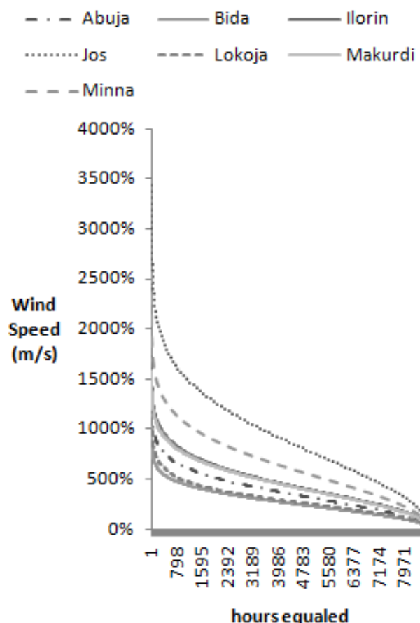
Fig.3. Plot of annual average hours equaled or exceeded for different wind speeds
