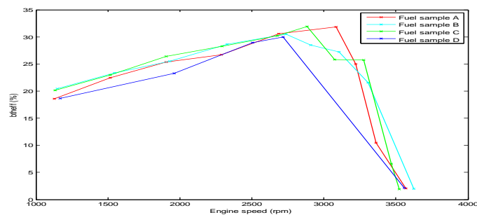
Figure 4.5: Brake thermal efficiency of the fuel samples
