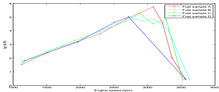
Figure 4.3: Brake power of the fuel samples.
