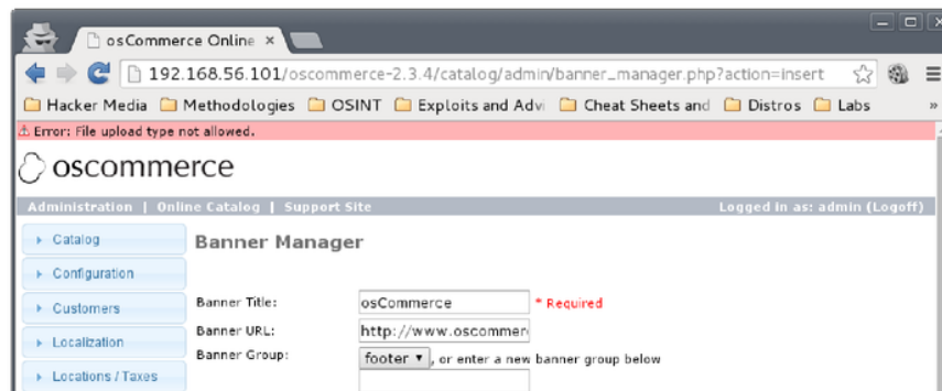
FIGURE 7. Warning file type not allowed.
