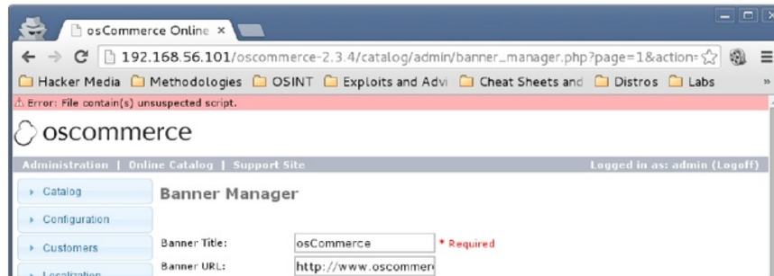
FIGURE 9. Warning content-type.
