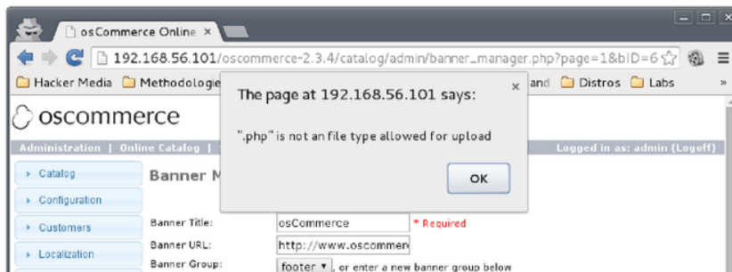
FIGURE 5. Alert javascript.
