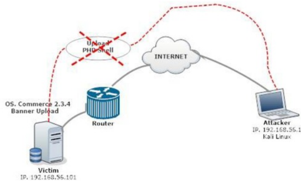
FIGURE 4. The process filter successfully.
