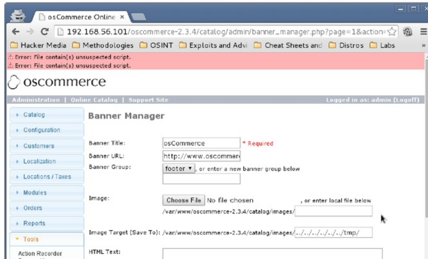
FIGURE 11. Warning input double dot
