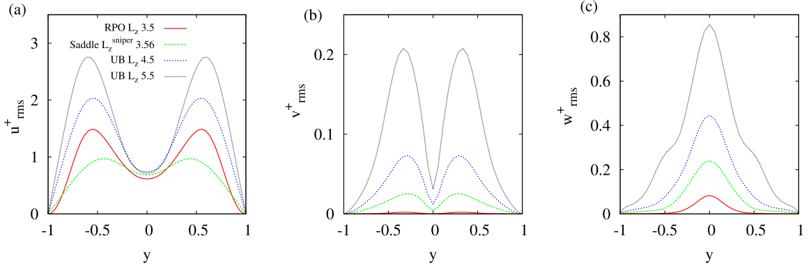
Fig. 7. Comparison of the rms velocity profiles of the travelling-wave upper branch solutions for selected values of L_z to the rms profiles of the relative periodic orbit solutions existing for L_z < L_z^* .
